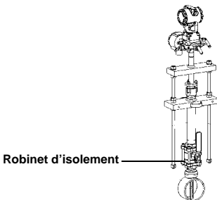
Figure 9. Installation du Flo-Tap
