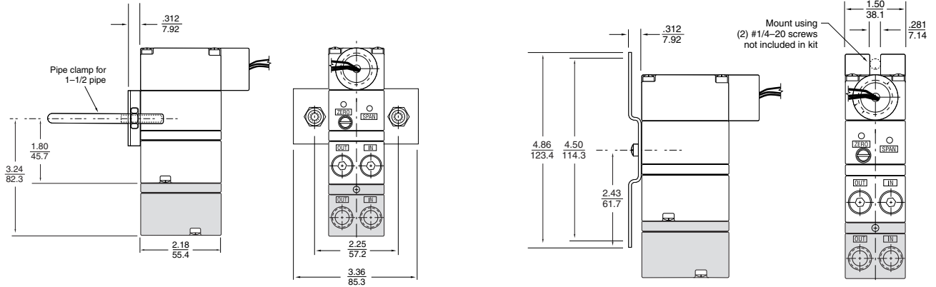
Figure 1 - Pipe Mounting Figure 2 - Panel Mounting
